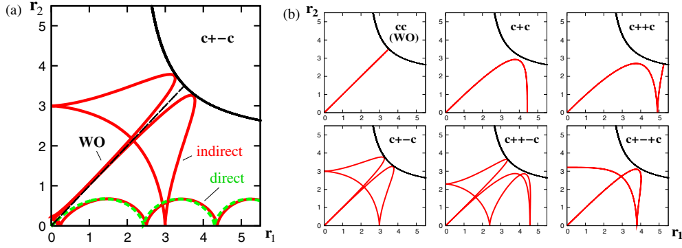
Figure 2. Triple collision dynamics and closed triple collision orbits: (a) trajectories starting near the triple collision point r_1 = r_2 = 0 and leading to ionization with fixed energy of the escaping electron; dashed (green) line: direct path; thick full (red) line: indirect path, here close to the CTCO c + -c ; (b) some short CTCOs together with binary symbol code.
