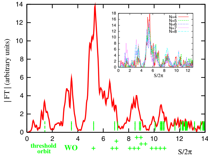
Figure 3. The Fourier spectrum of the fluctuating part of the partial cross section in figure 1 averaged over N = 4 - 8 ; the actions of CTCOs are marked on the axis together with their respective binary symbol code. Inset: individual Fourier signals.
