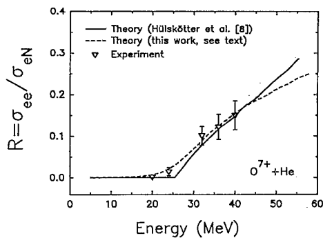
FIG. 4. The ratio of cross sections for the ee ( \sigma_{ee} ) and eN ( \sigma_{eN} ) processes as deduced from the present data is shown as open triangles. Theoretical curves are from Hülskötter et al. [8] (solid line) and from a calculation described in the text (dashed line).
