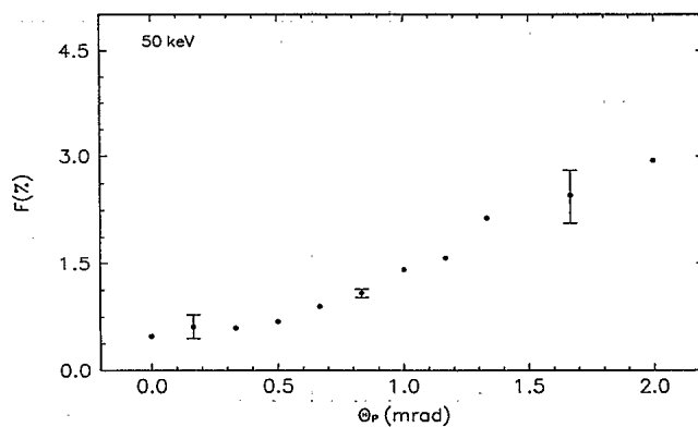
FIG. 4. The ratio of the transfer ionization to total capture events as a function of the laboratory scattering angle for a 50-keV proton-helium collision. Error bars represent the standard deviation of the mean from all the data sets.
