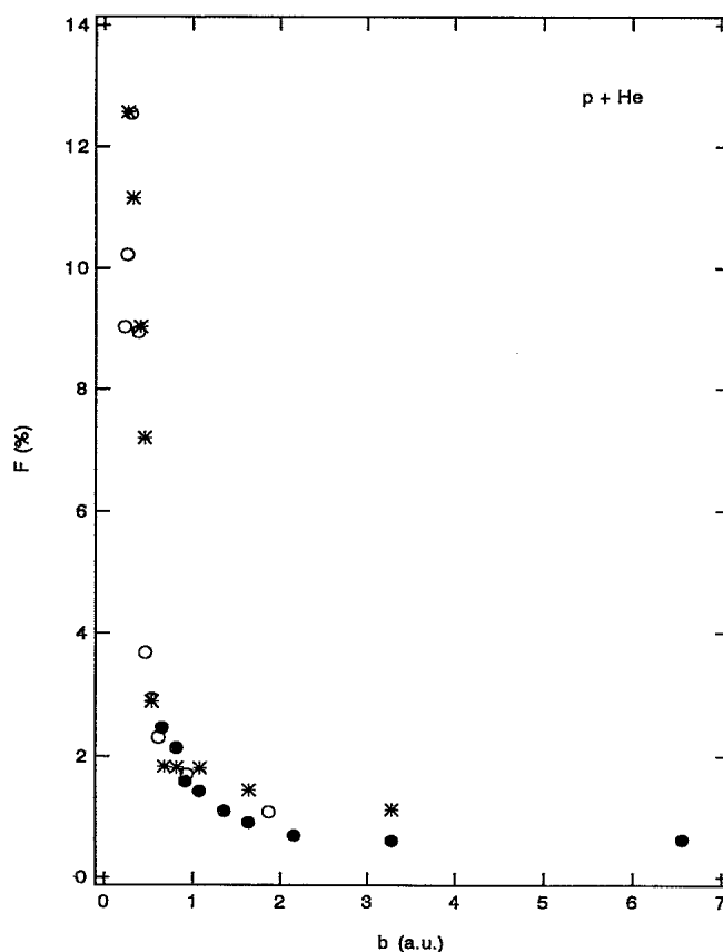
FIG. 7. The ratio of transfer ionization to total capture as a function of the impact parameter. The full circles are the data for 50 keV, the stars for 100 keV, and the open circles for 175 keV.
