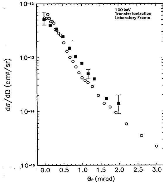
FIG. 10. Same as Fig. 9 for 100 keV.
