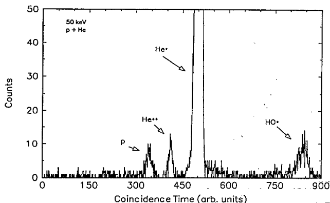
FIG. 2. A coincidence time spectrum taken for a collision energy of 50 keV and a scattering angle of 0^\circ . Besides the \text{He}^+ and \text{He}^{2+} recoil ions, protons and \text{HO}^+ ions can be identified which are due to water vapor in the residual gas.
