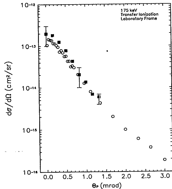
FIG. 11. Same as Fig. 9 for 175 keV.
