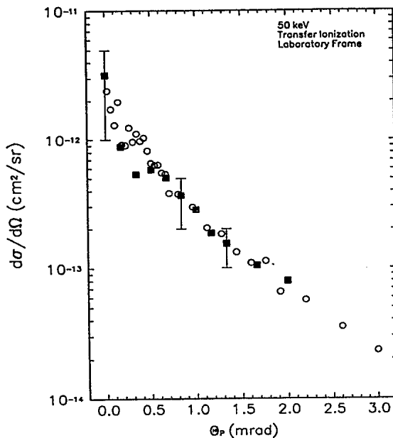
FIG. 9. Differential transfer ionization cross sections as a function of laboratory scattering angle for 50-keV p + \text{He} . The squares are the experimental data, the open circles show a dCTMC calculation by Meng and Olson [15].
