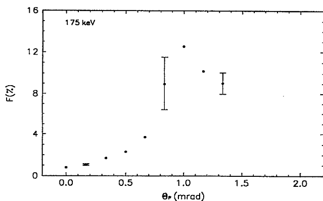
FIG. 6. Same as Fig. 4 for 175 keV.
