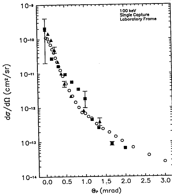
FIG. 8. Differential single-capture cross sections as a function of laboratory scattering angle for 100-keV p + \text{He} . The squares are the experimental data of this work, the triangles are experimental data from Martin et al. [10], and the open circles show a dCTMC calculation by Meng and Olson [15].
