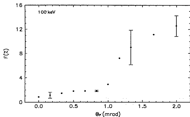
FIG. 5. Same as Fig. 4 for 100 keV.
