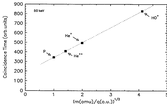
FIG. 3. Plot of the coincidence time vs the square root of the mass to charge ratio of the recoil ions. The linear dependence indicates a correct assignment of the recoil ion species to the time peaks in Fig. 2.
